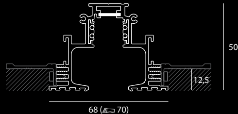
type 2 RA 12.5 mm / 15 mm / 18 mm
