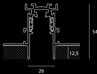
type 2 RC / 12.5 mm
