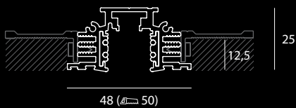
type 1 RA 12.5 mm / 15 mm / 18 mm
