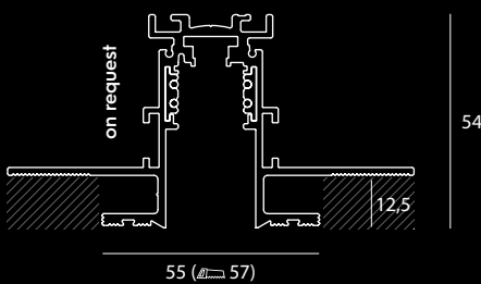
type 1 RA 12.5 mm / 15 mm / 18 mm
